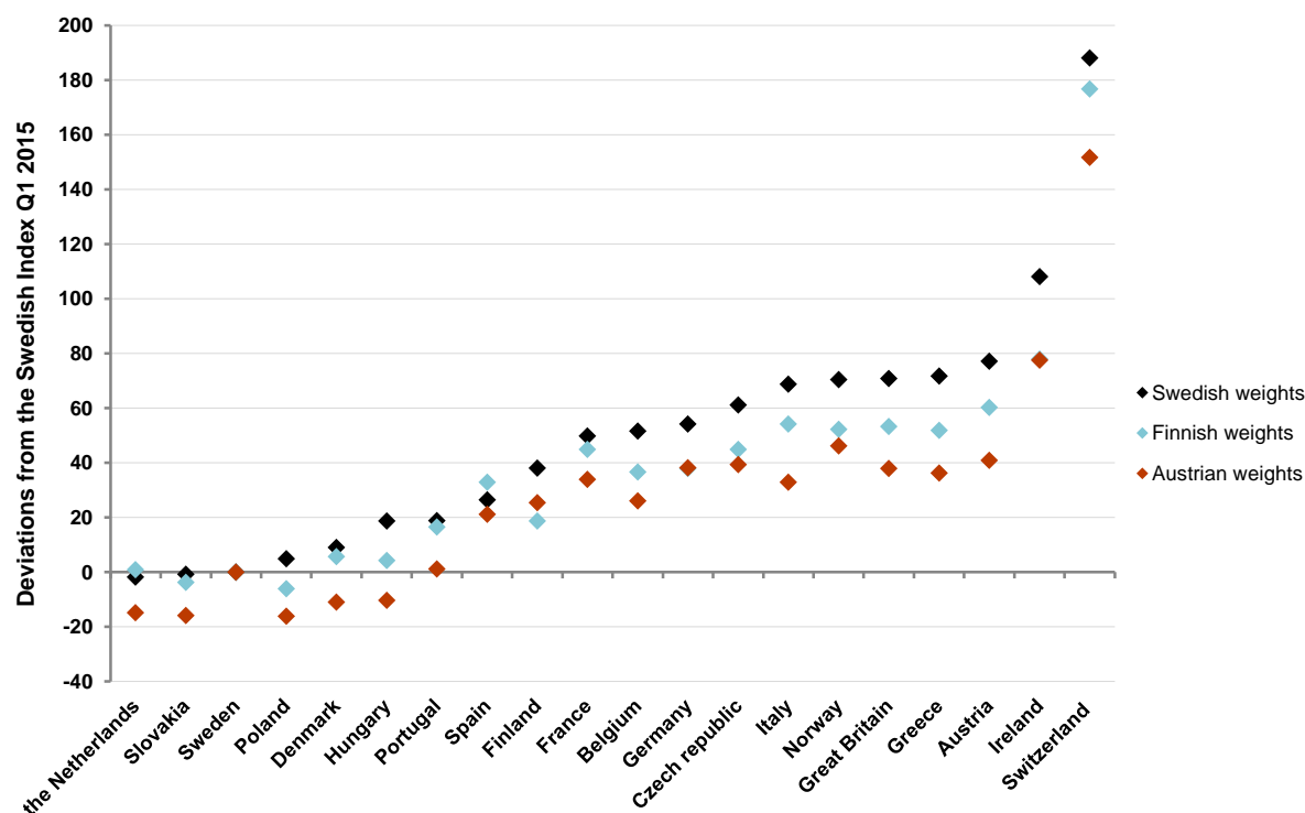
Figure 19. The bilateral price indices with Swedish, Finnish and Austrian sales volumes and volume weights, and relative deviations from the Swedish index, Q1 2015, for the segment pharmaceuticals with competition.
